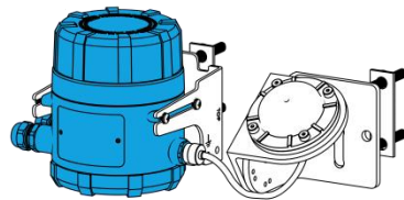
Figure 2. Inclinometer using 2" pole U-bolt
