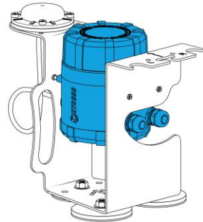
Figure 1. Inclinometer using a floating roof mounting bracket with magnetic feet
